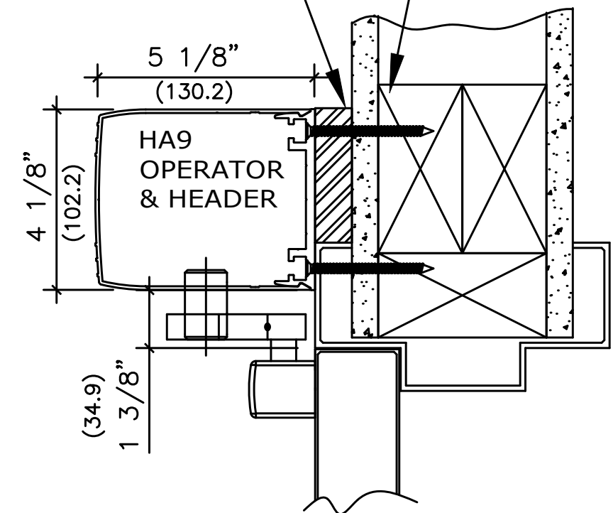
VERTICAL SECTION
