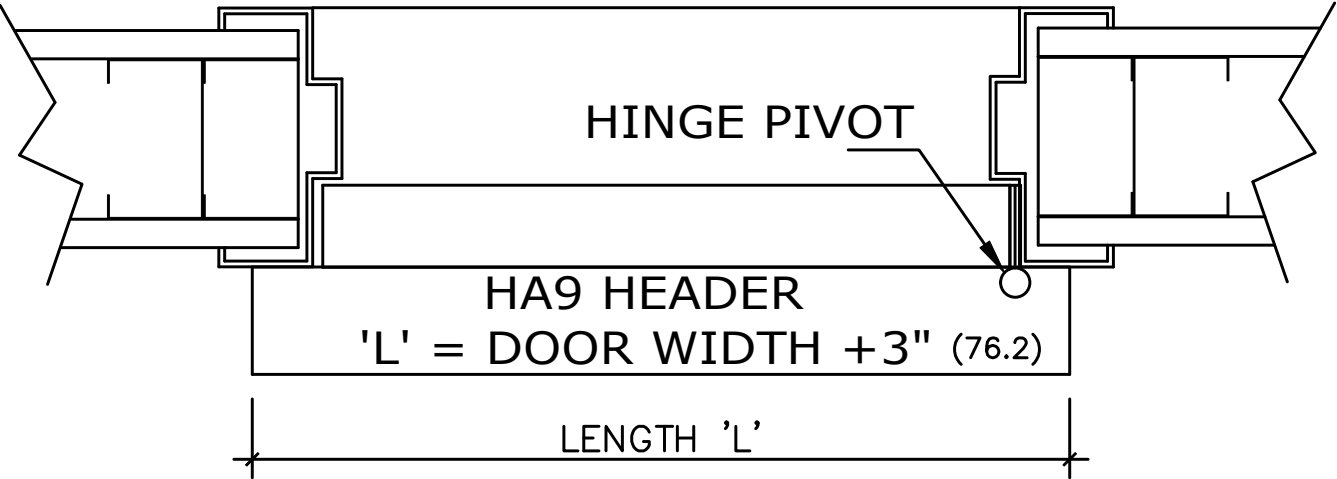
INTERIOR HORIZONTAL SECTION
