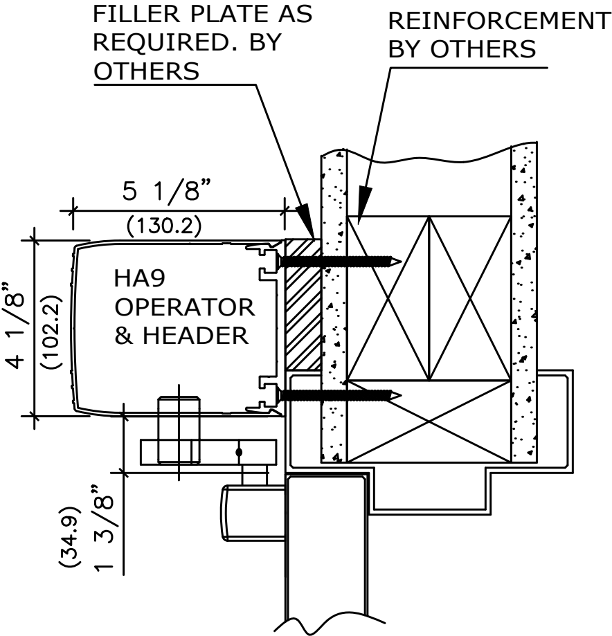
VERTICAL SECTION
