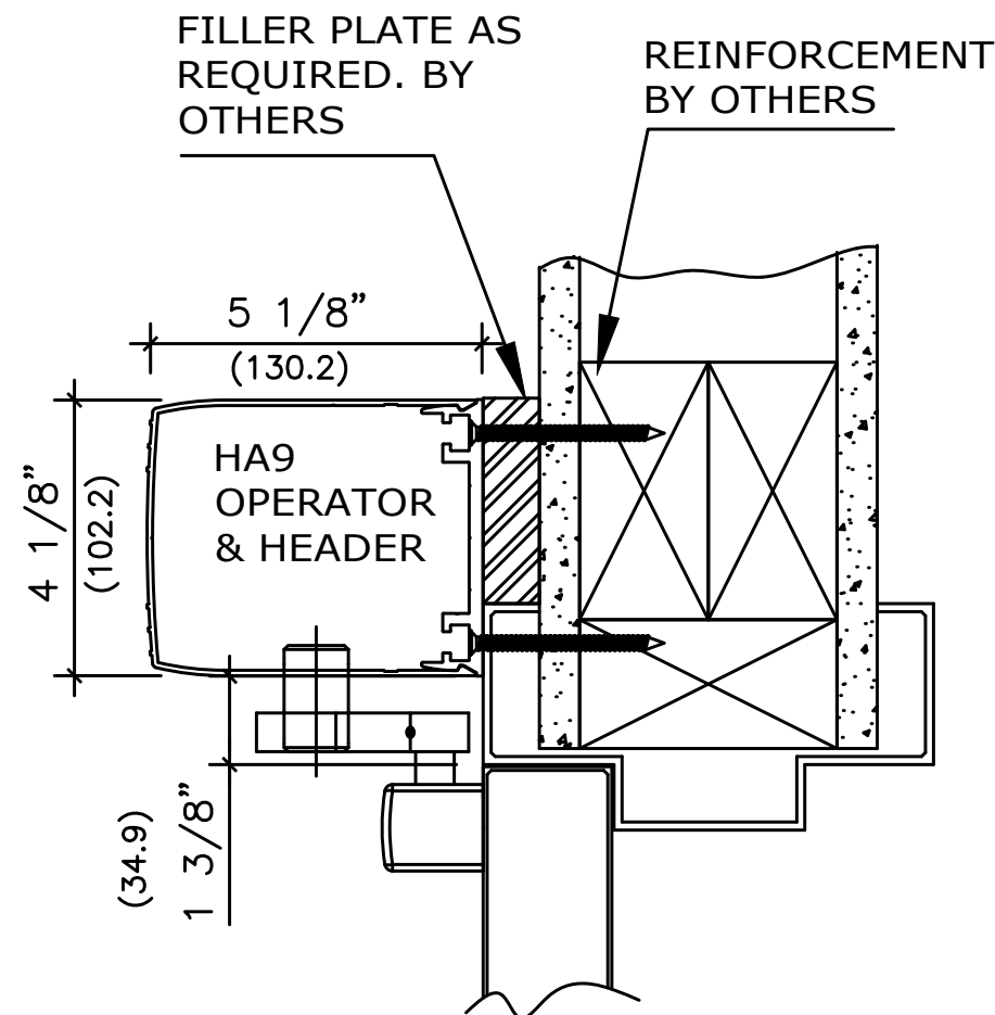
VERTICAL SECTION
