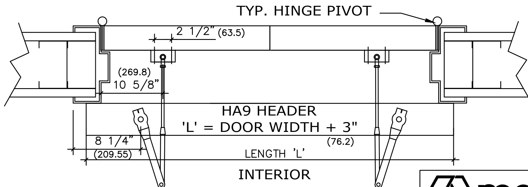
HORIZONTAL SECTION
