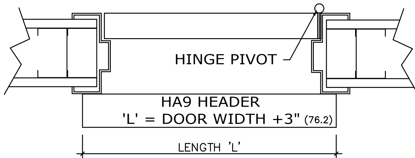
INTERIOR HORIZONTAL SECTION
