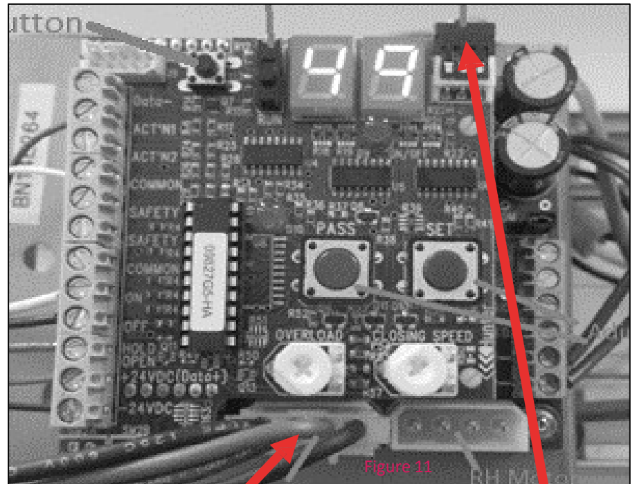
Motor Connection
