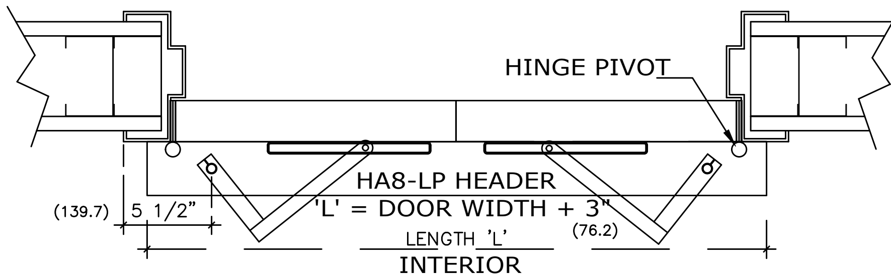
HORIZONTAL SECTION
