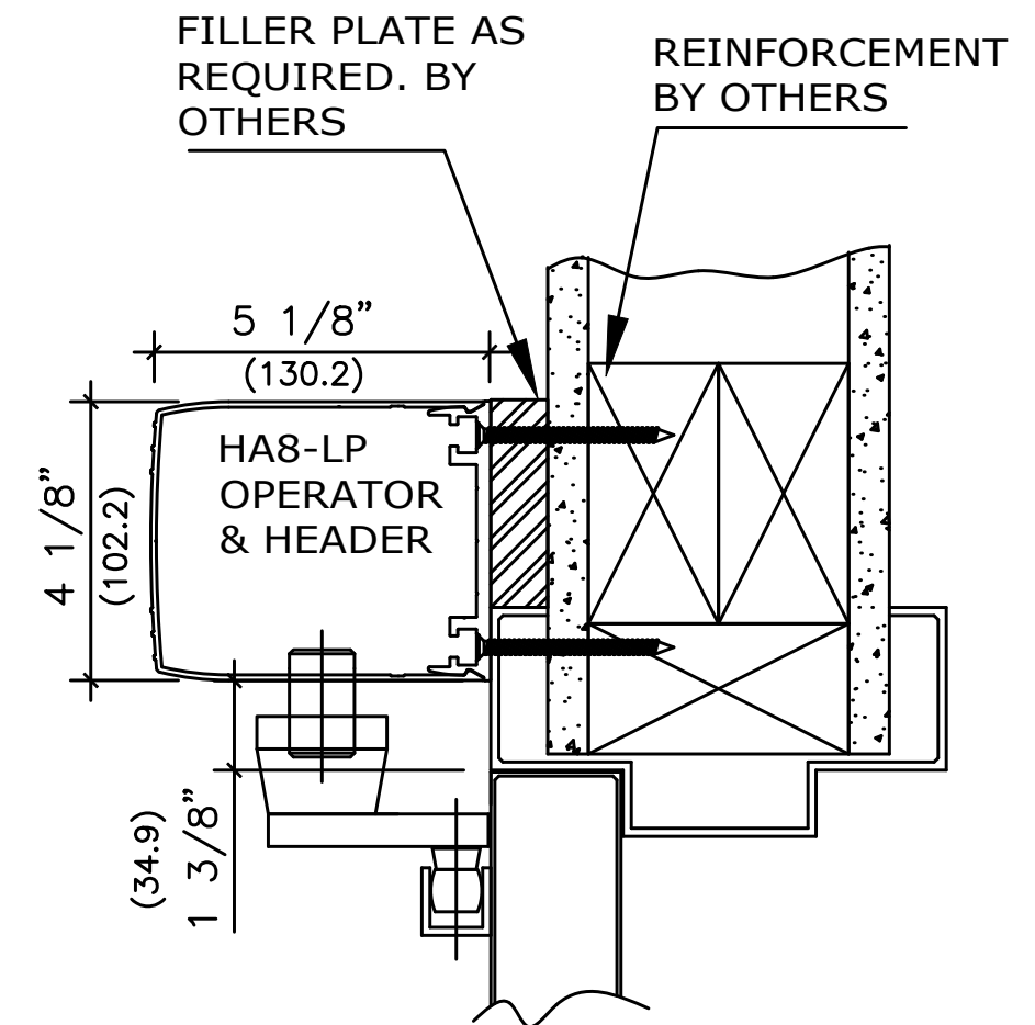
VERTICAL SECTION
