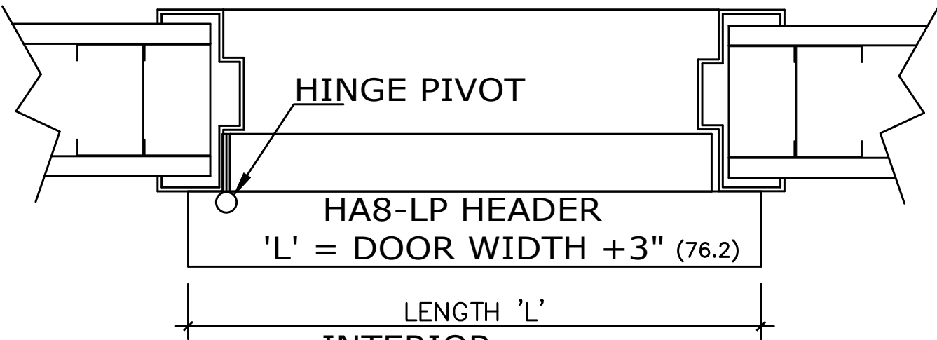
INTERIOR HORIZONTAL SECTION
