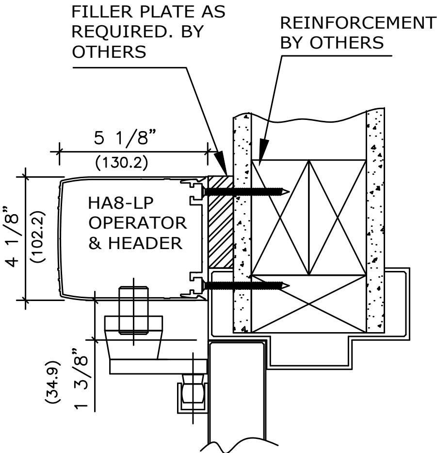
VERTICAL SECTION
