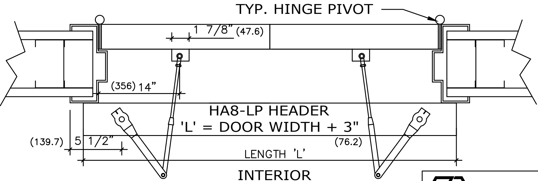
HORIZONTAL SECTION
