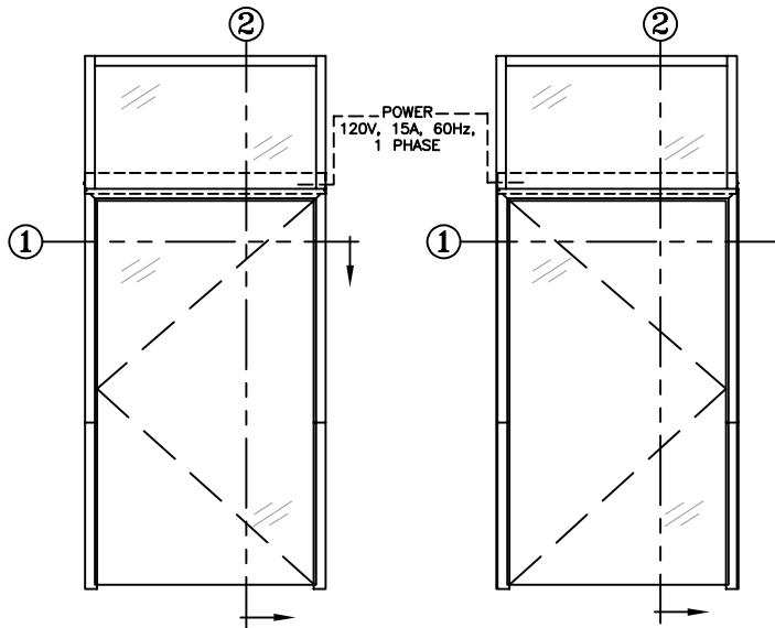
ELEVATION VIEW
