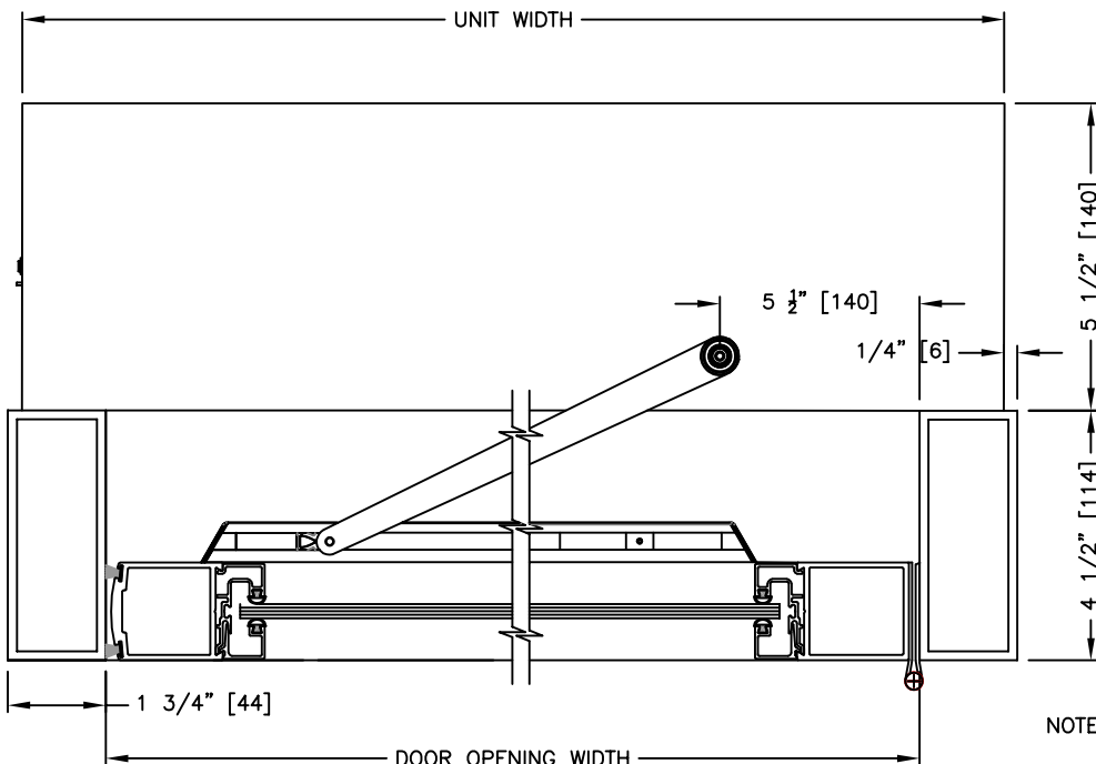
SECTION: 1
