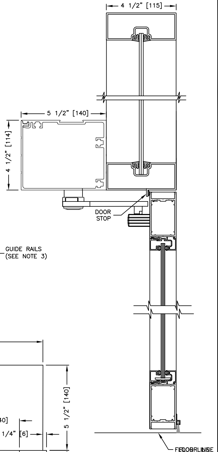
SECTION: 2
