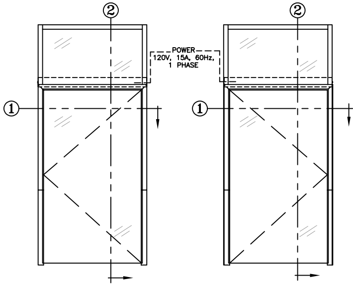
ELEVATION VIEW
