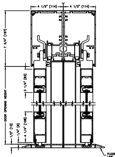
SECTION: 2
