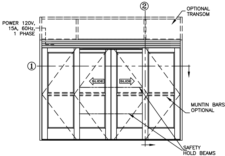
ELEVATION VIEW
