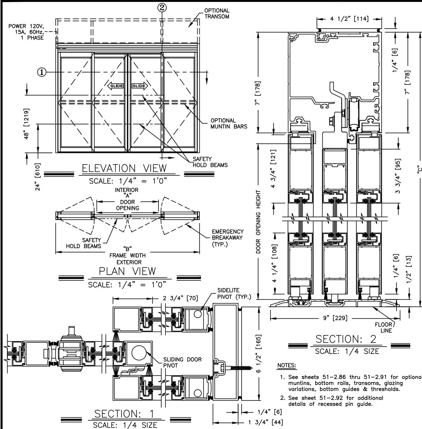
DIMENSIONS FOR STANDARD NARROW STILE PACKAGES
