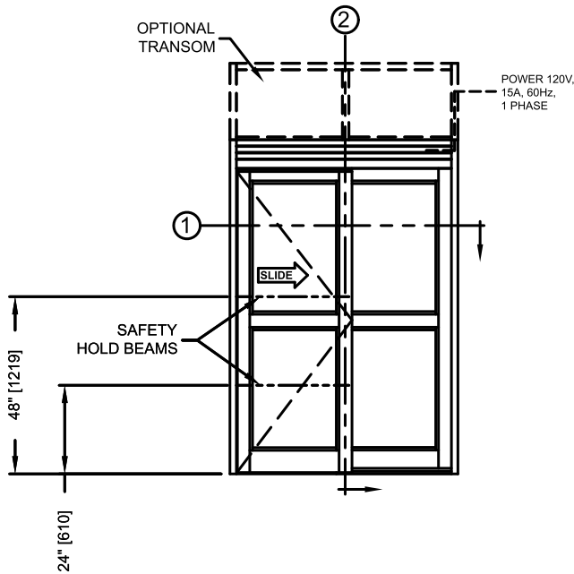
ELEVATION VIEW
