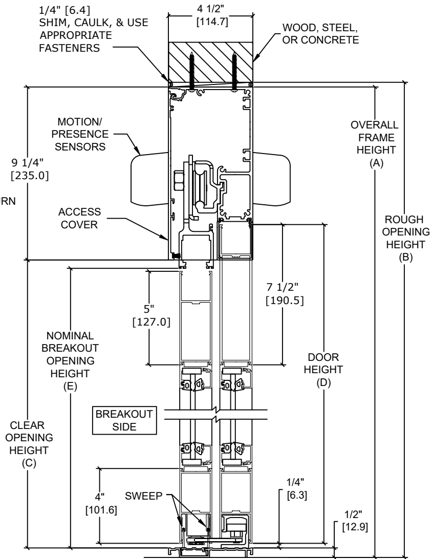
SECTION B-B SCALE - 1:1
