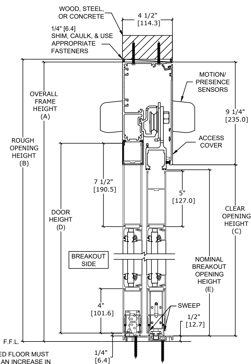
SECTION B-B
