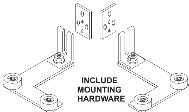
4-56-0001 - LH BOTTOM GUIDE ASSY. WOOD DBO
