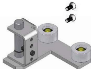
4-11-0471 RH Sway Guide Assembly
