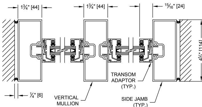
HORIZONTAL SECTION THROUGH TRANSOM (SHOWN WITH 5/8" THERMAL GLAZING)
