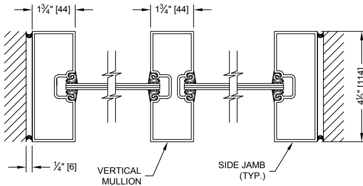
HORIZONTAL SECTION THROUGH TRANSOM (SHOWN WITH 1/4" GLAZING)
