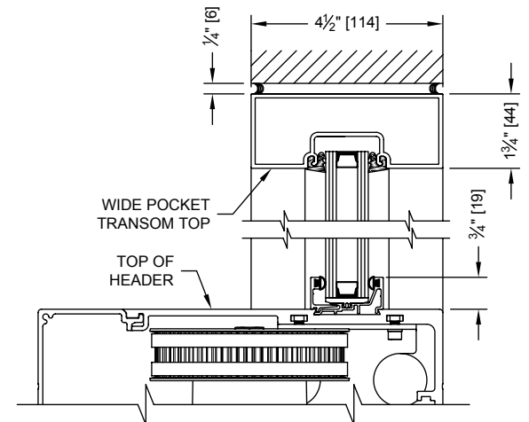
VERTICAL SECTION THROUGH TRANSOM (SHOWN WITH 1" THERMAL GLAZING)
