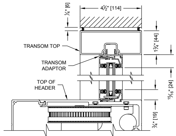
VERTICAL SECTION THROUGH TRANSOM (SHOWN WITH 5/8" THERMAL GLAZING)
