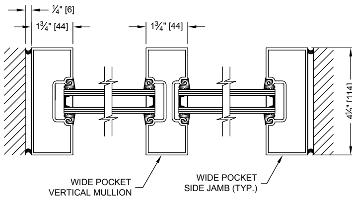
HORIZONTAL SECTION THROUGH TRANSOM (SHOWN WITH 1" THERMAL GLAZING)
