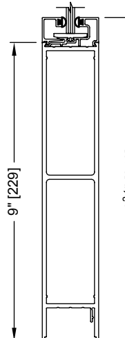
9" TALL BOTTOM RAIL
