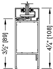
3 1 / 2 " BOTTOM RAIL
