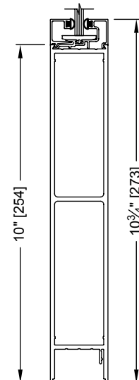
10" TALL BOTTOM RAIL
