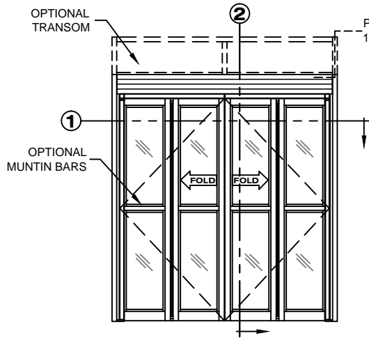
ELEVATION VIEW
