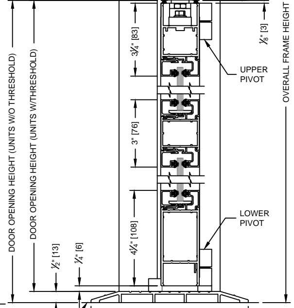
SECTION: 2
