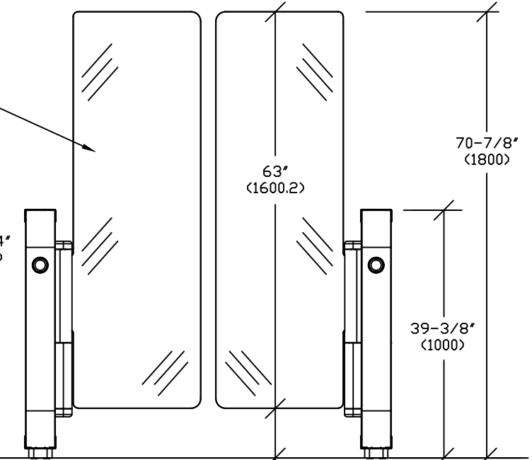
FRONT VIEW HIGH GLASS
