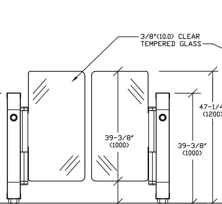
FRONT VIEW MID GLASS
