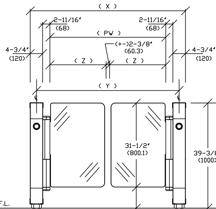
FRONT VIEW LOW GLASS
