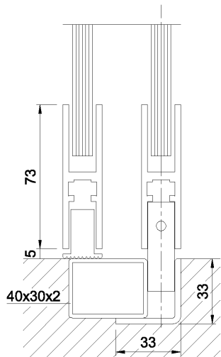
Substructure
