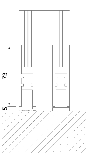
Floor guide
