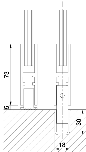
Floor track
