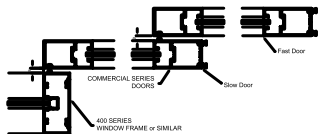
HANGER CHANNEL FIXING
