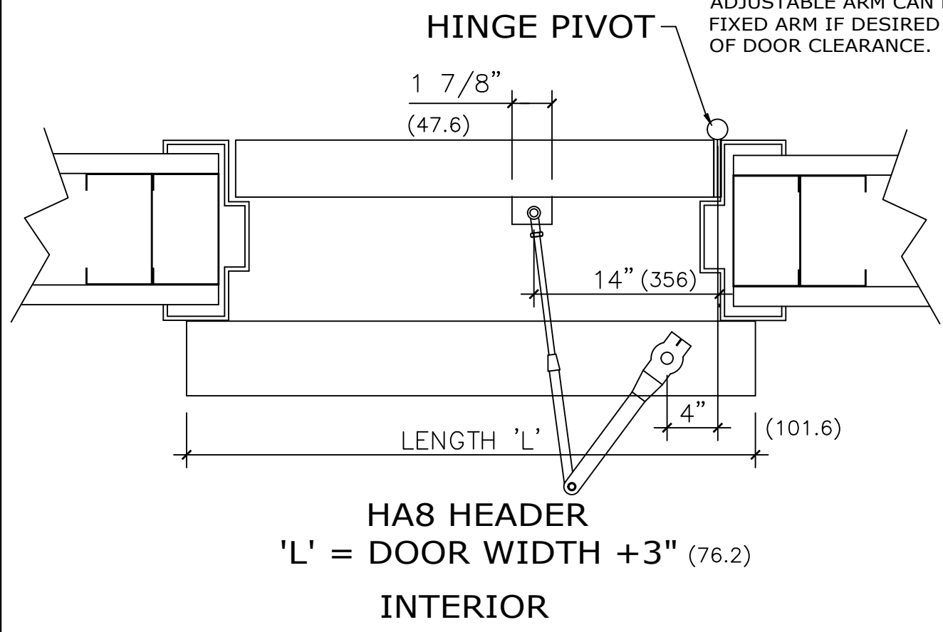
2 HORIZONTAL SECTION
