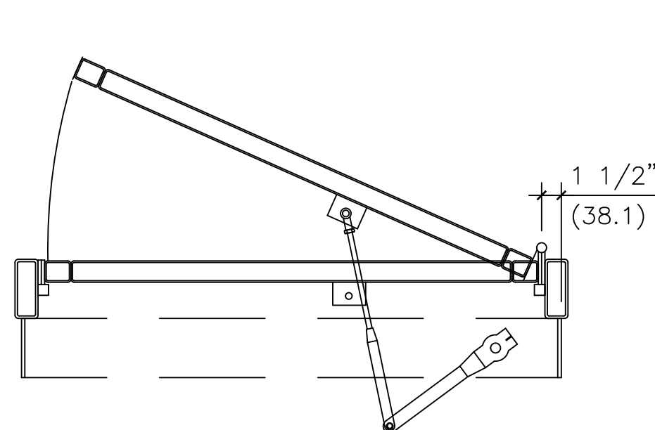
INTERIOR PLAN
