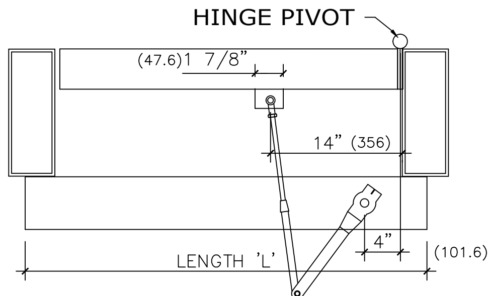
HA8 HEADER 'L' = DOOR WIDTH + 3" (76.2) INTERIOR
