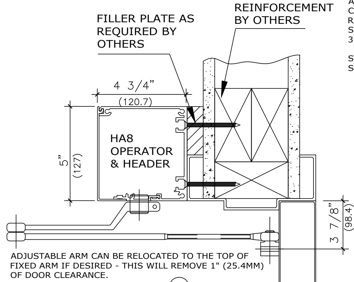
VERTICAL SECTION
