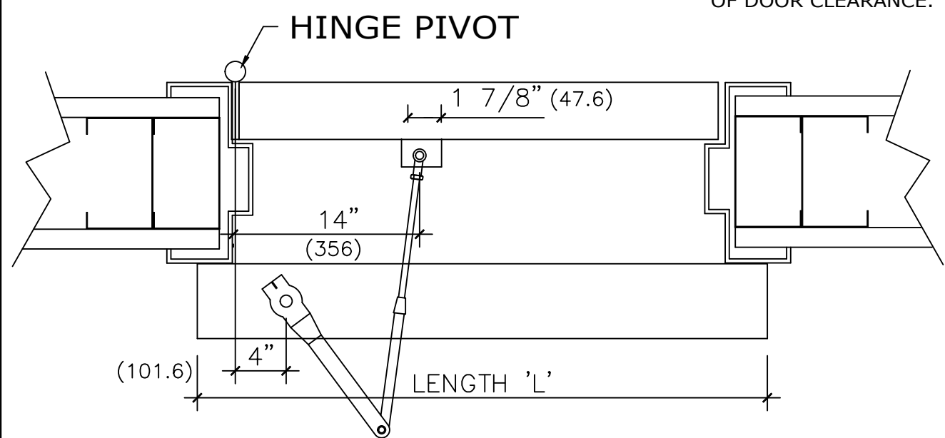
HA8 HEADER 'L' = DOOR WIDTH + 3" (76.2) INTERIOR
