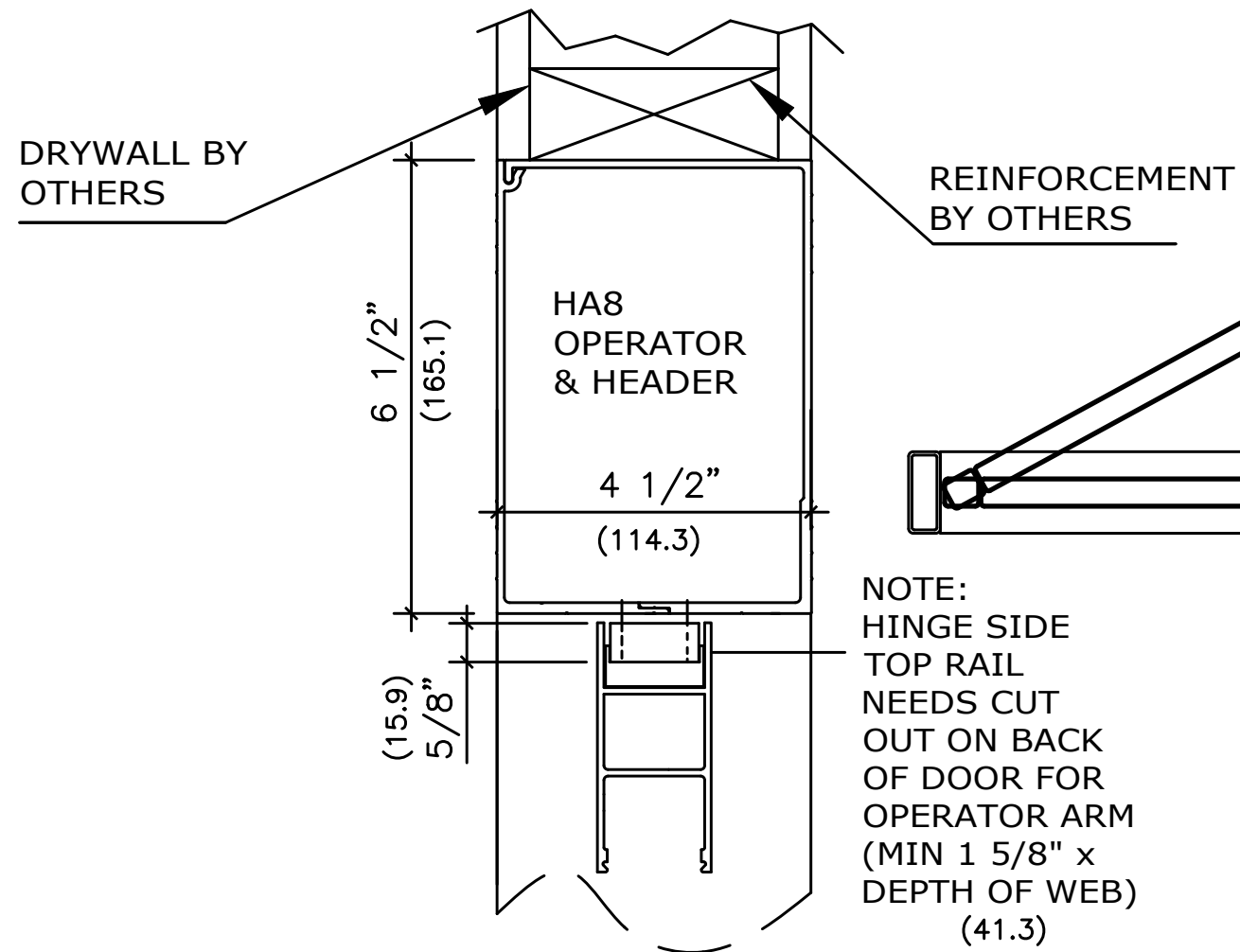
VERTICAL SECTION
