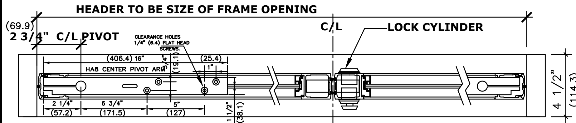
INTERIOR HORIZONTAL SECTION
