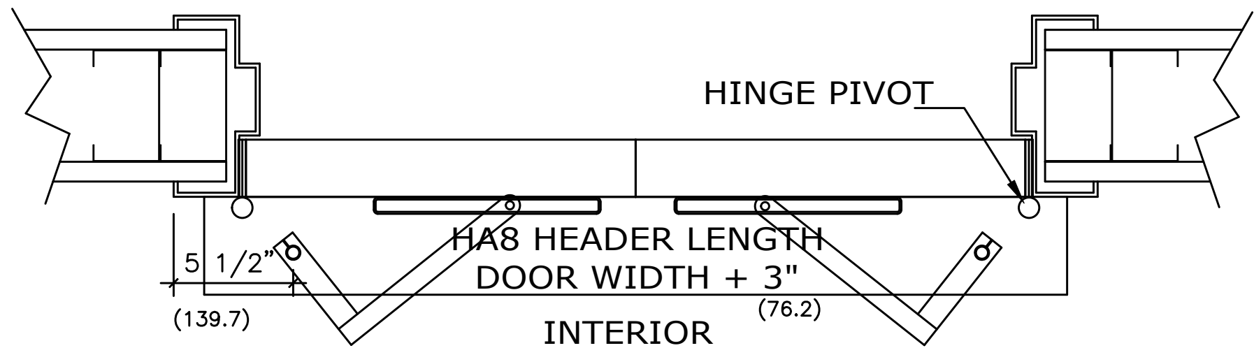
HORIZONTAL SECTION
