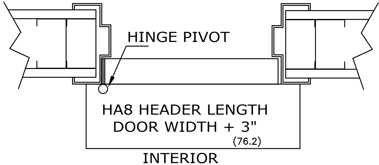
HORIZONTAL SECTION
