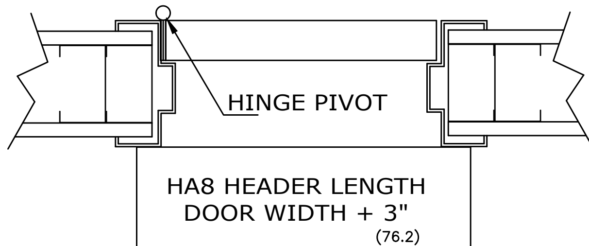
HORIZONTAL SECTION
