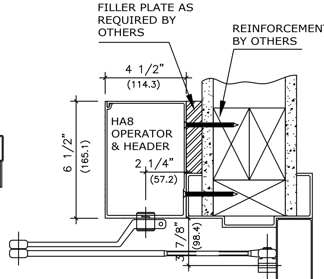
VERTICAL SECTION
