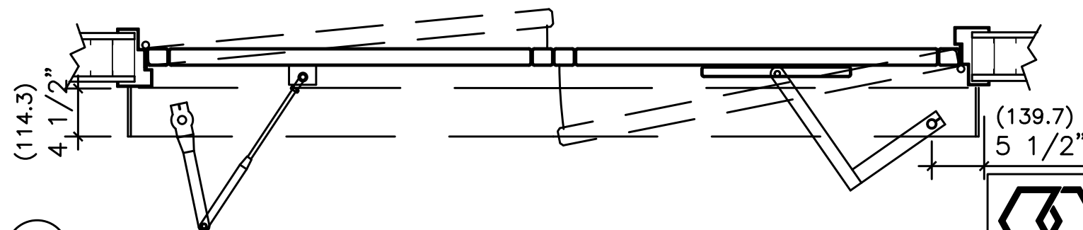
3 HORIZONTAL SECTION
