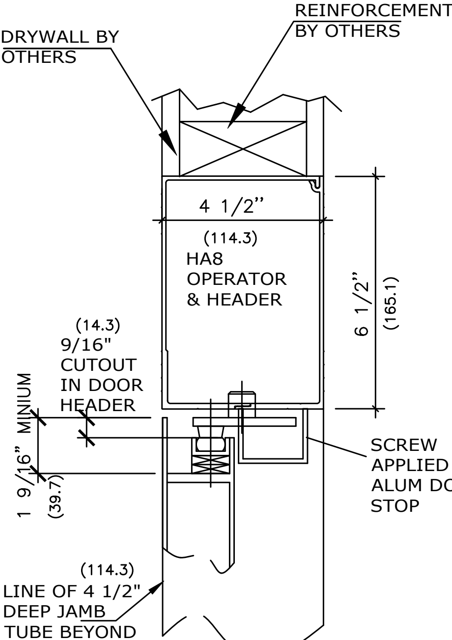
VERTICAL SECTION
