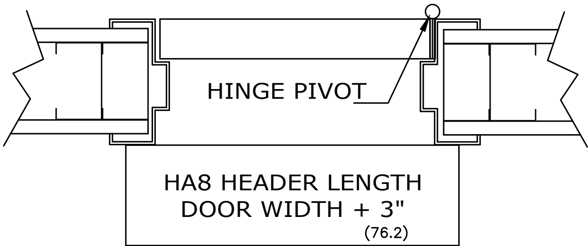
INTERIOR HORIZONTAL SECTION
