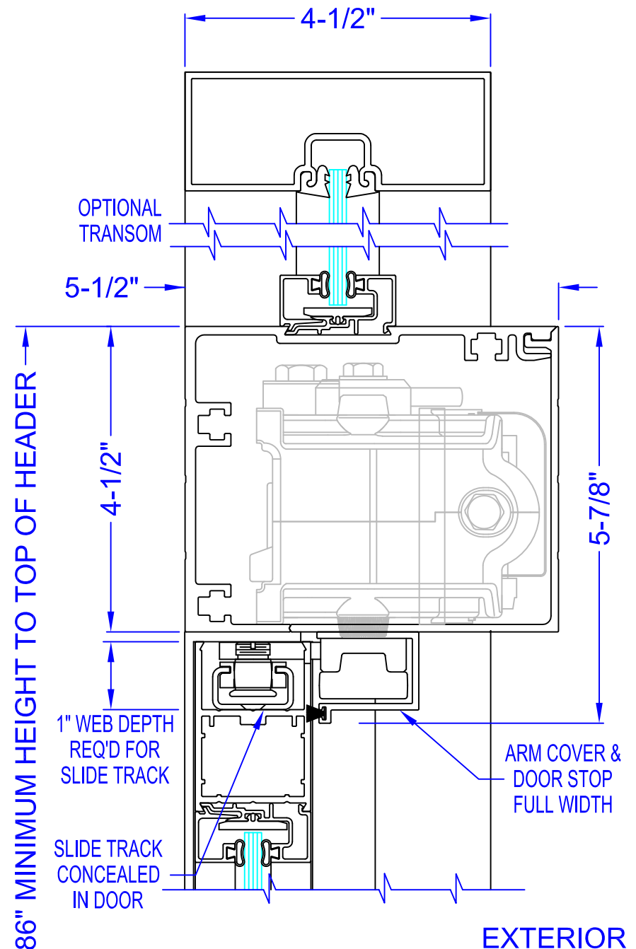
HEAD SECTION SCALE: 1/2 SIZE
